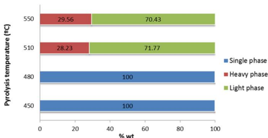
Figure 3: Bio-oil quality after the fast pyrolysis experiments.
