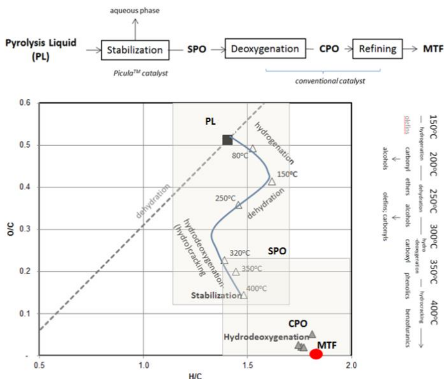
Figure 1: Van Krevelen plot for pyrolysis oil and hydrotreated products at several maximum induced bed temperatures (MIBT).
