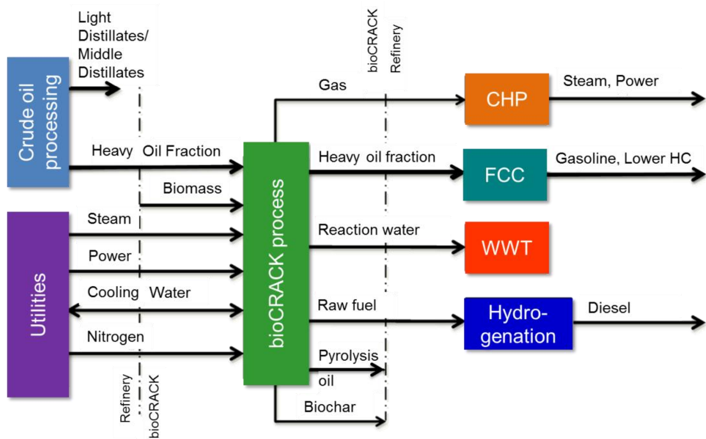
Figure 2: Process flow sheet of the bioCRACK refinery integration concept.
